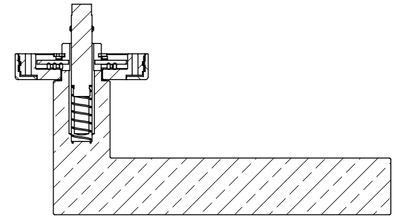
SECTION F-F
